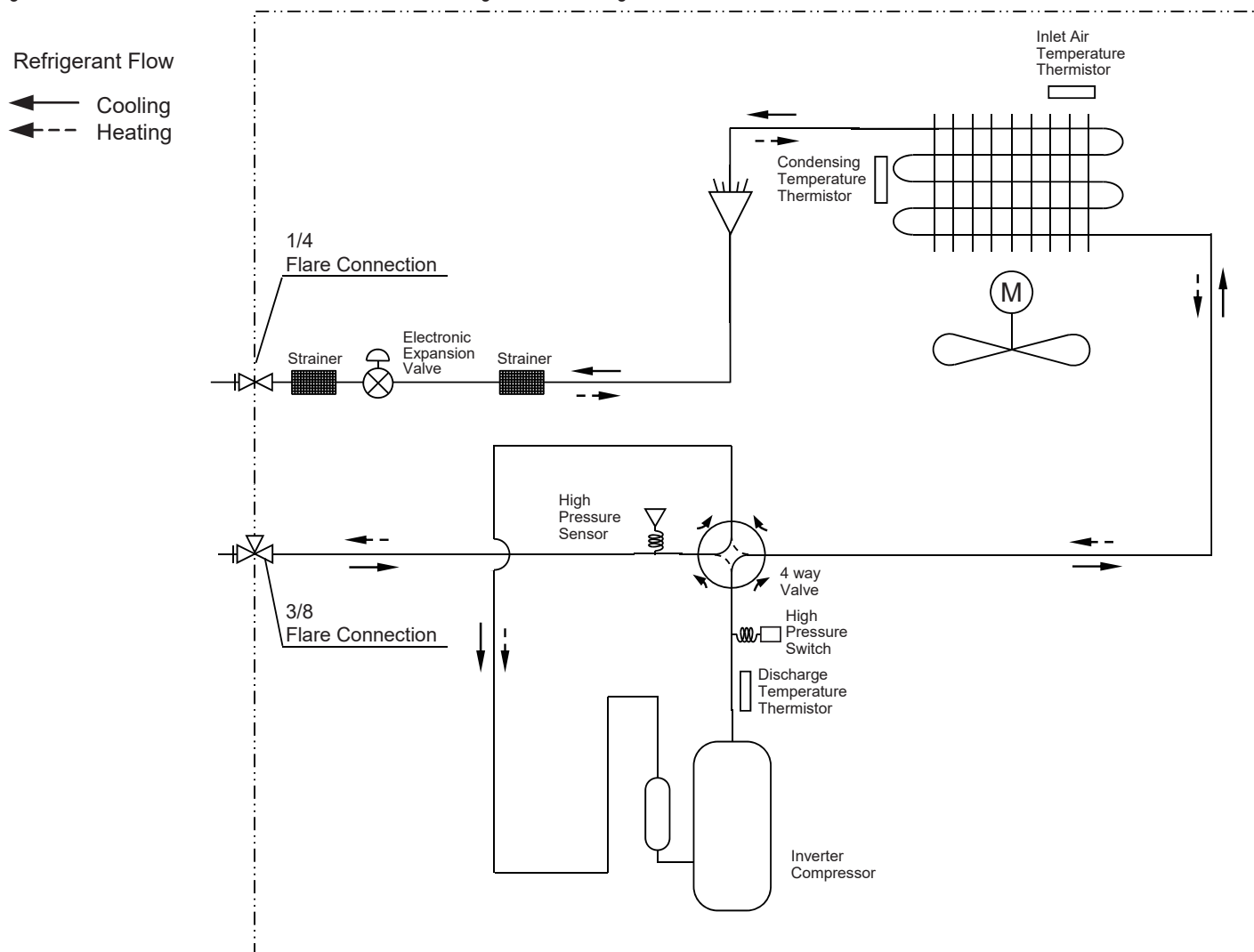
Figure 43: KUSXB091A, KUSXB121A Outdoor Unit Refrigerant Flow Diagram.
