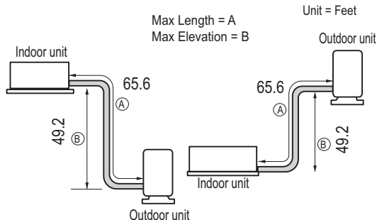
Figure 51: Typical KSSCB361A, KSSCB421A, KSSCB481A System Layout.
