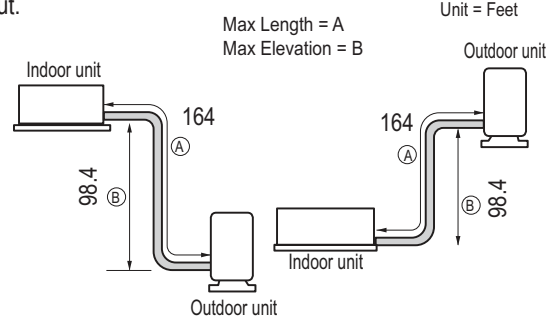
Figure 50: Typical KSUDB181A, KSSCB241A, and KSSCB301A System Layout.
