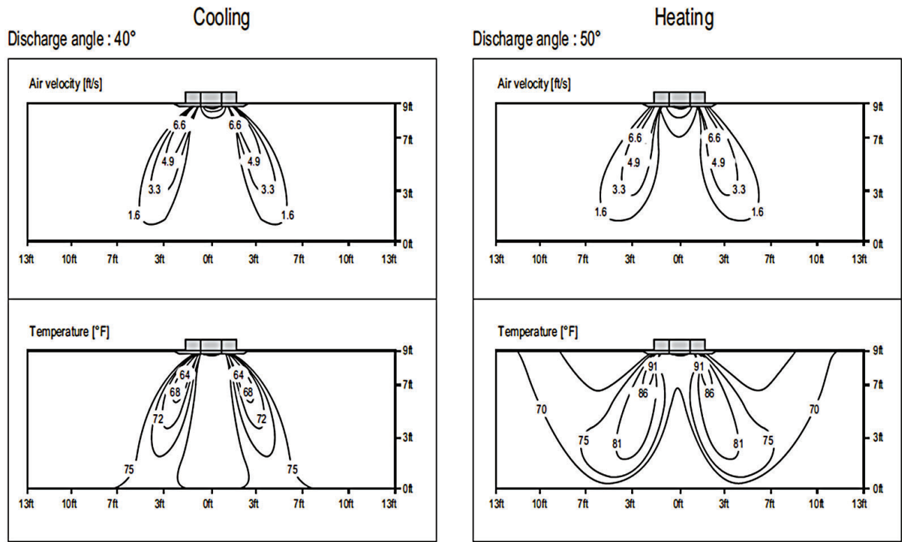
Figure 16: KNUDB181A Air Velocity and Temperature Distribution Charts.
