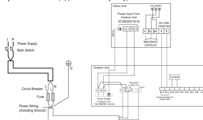
Figure 66: General R32 Single-Zone System Power / Communications System Schematic (Appearances May Vary).
