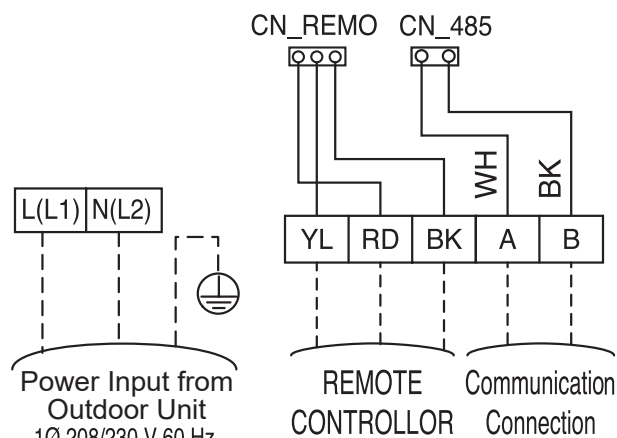
Figure 71: Wired Controller Connection (Example Only).
