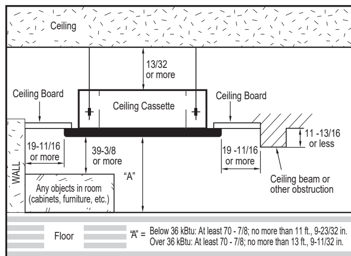
Figure 26: Cassette Indoor Unit Clearance Requirements.
