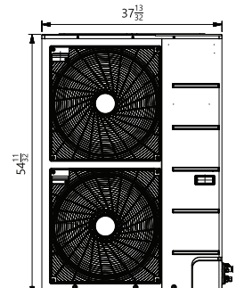
Outdoor Unit Dimensions
