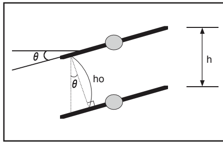
Figure 41: Open Rate by Louver Radian Formula.
