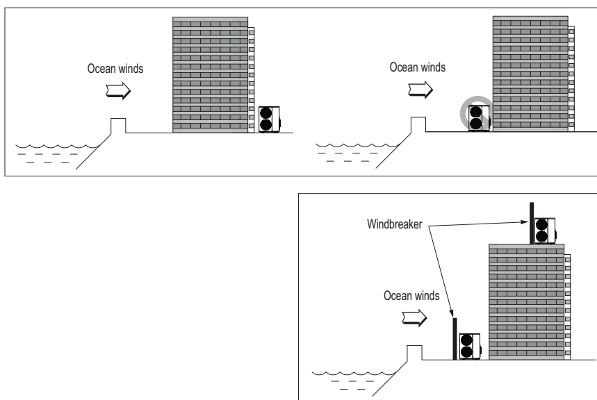
Figure 34: Oceanside Placement Using a Building as Shield, and Placement Using a Windbreak.
