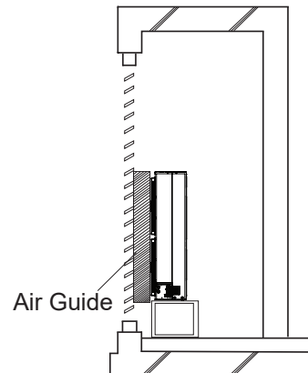
Air Guide Duct on Outdoor Unit
