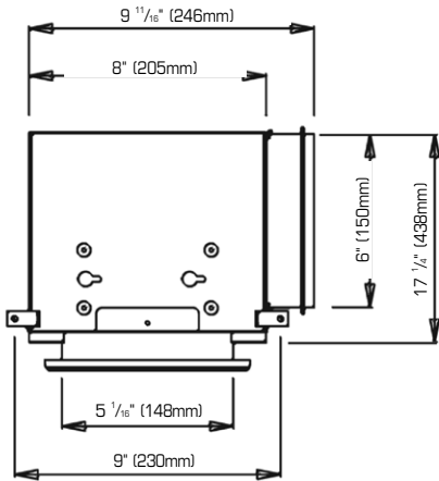
Housing Dimensions of 6" duct models
