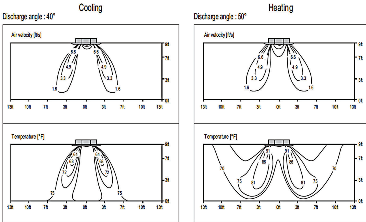
Figure 12: KNUDB181A Air Velocity and Temperature Distribution Charts.
