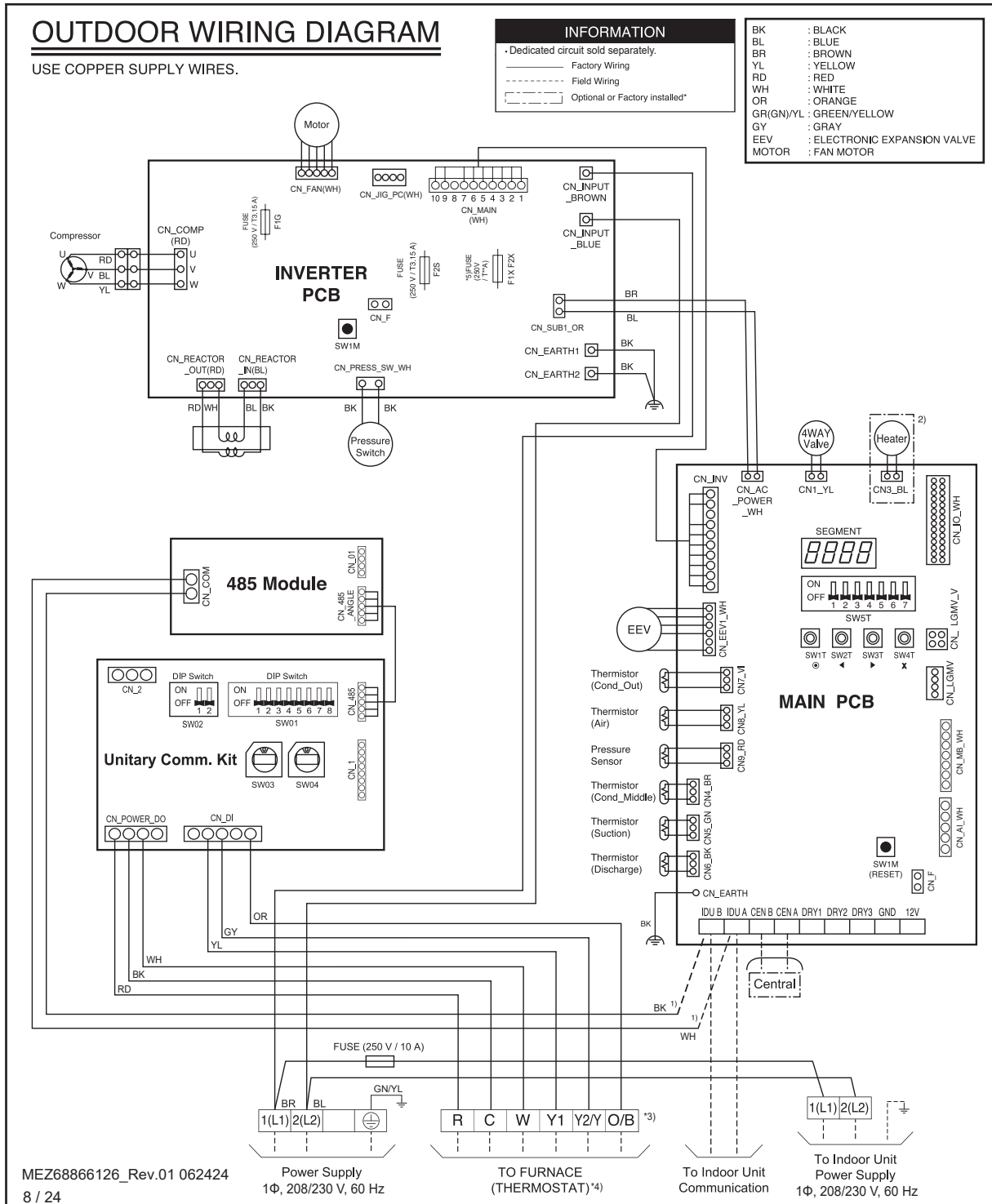
Figure 52: KUSXA181A, KUSXA241A Outdoor Unit Wiring Diagram.
