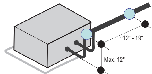
Figure 50: Pipe Support at Indoor Unit.
