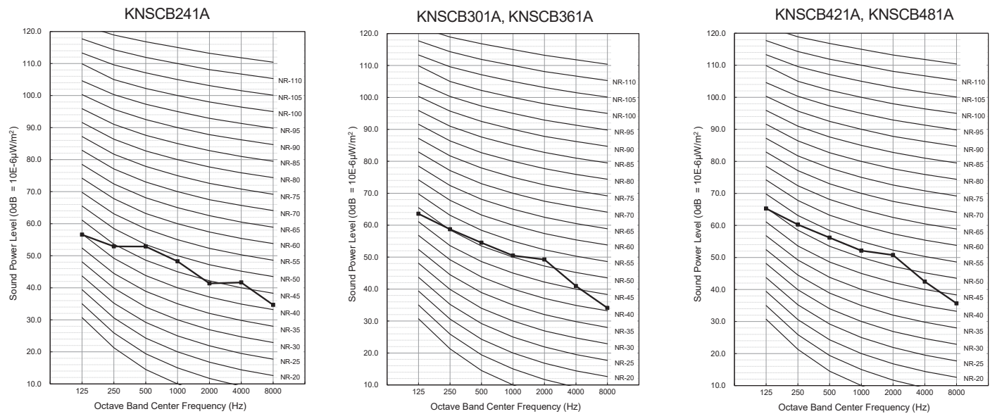
Figure 21: LGRED Four-Way Cassette Indoor Unit Sound Power Level Diagrams.
