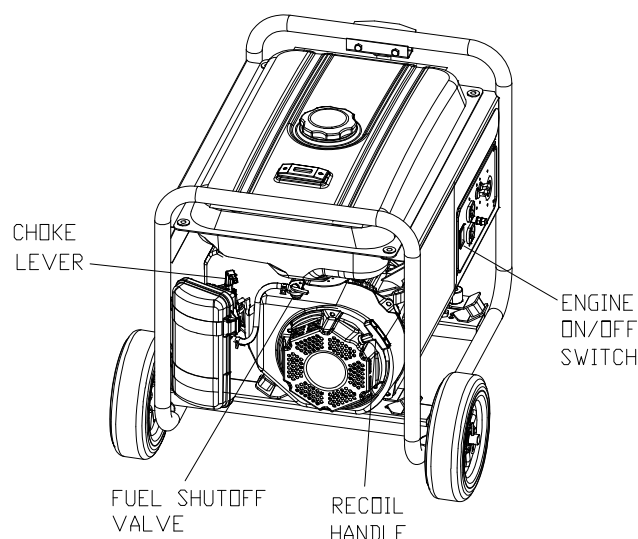
Figure 11 - Engine Controls
