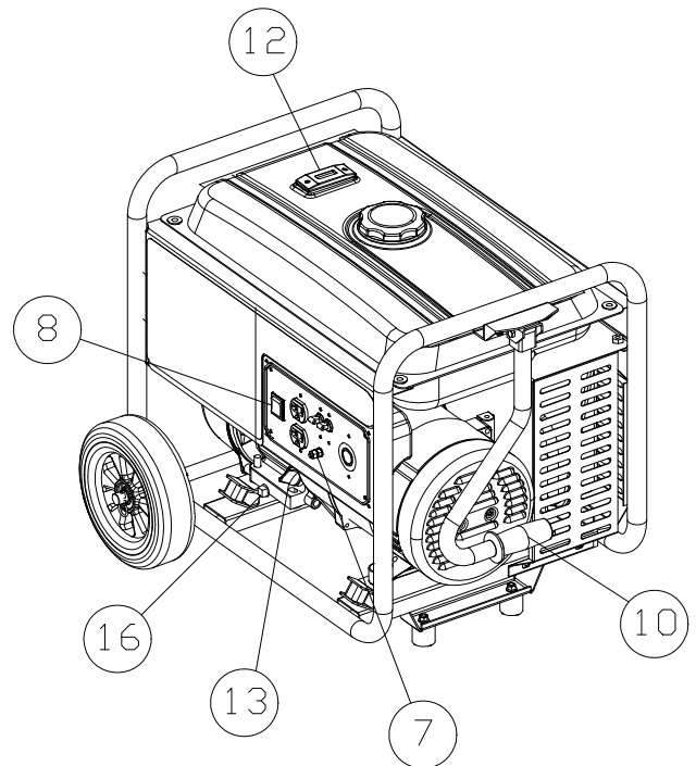
Figure 5 - Generator Controls
