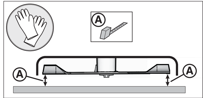
Figure 40. Measuring the Blade Height
