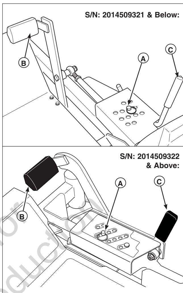
Figure 6. Mowing Height Adjustment
