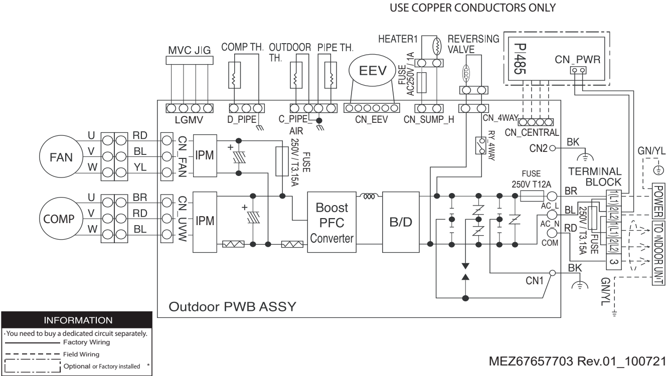
Figure 22: Wiring Diagram for LSU090HSV5, LSU120HSV5 Units.
