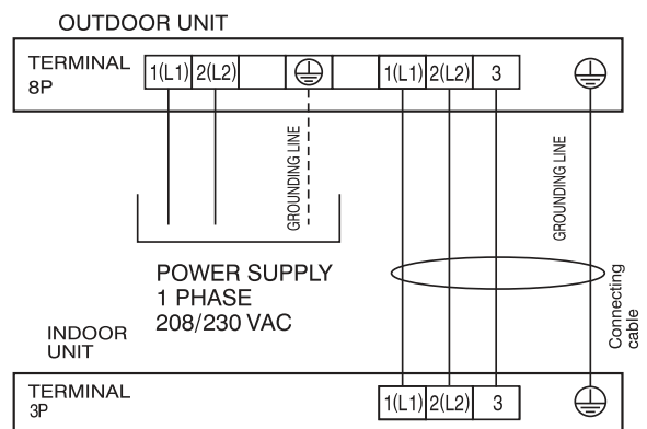
Figure 27: LA181HSV5 System Electrical Connections.
