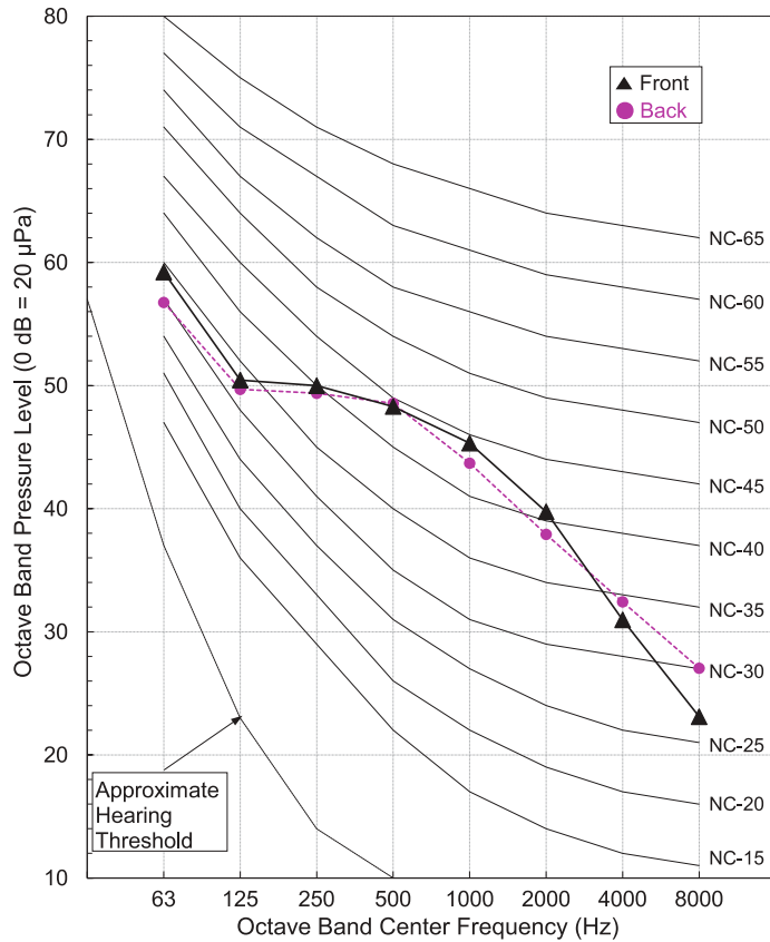
Figure 17: LSU181HSV5 Cooling Sound Pressure Level Diagram.
