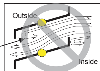
Figure 43: Using “S” Type Louvers.
