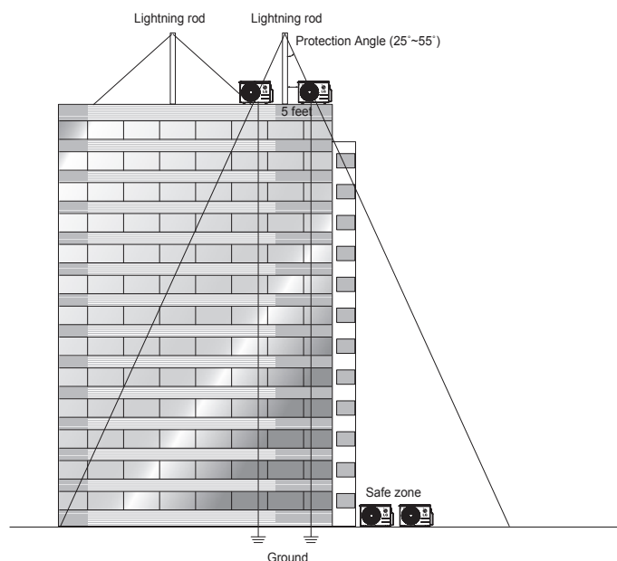
Figure 38: Lightning Protection Diagram.
