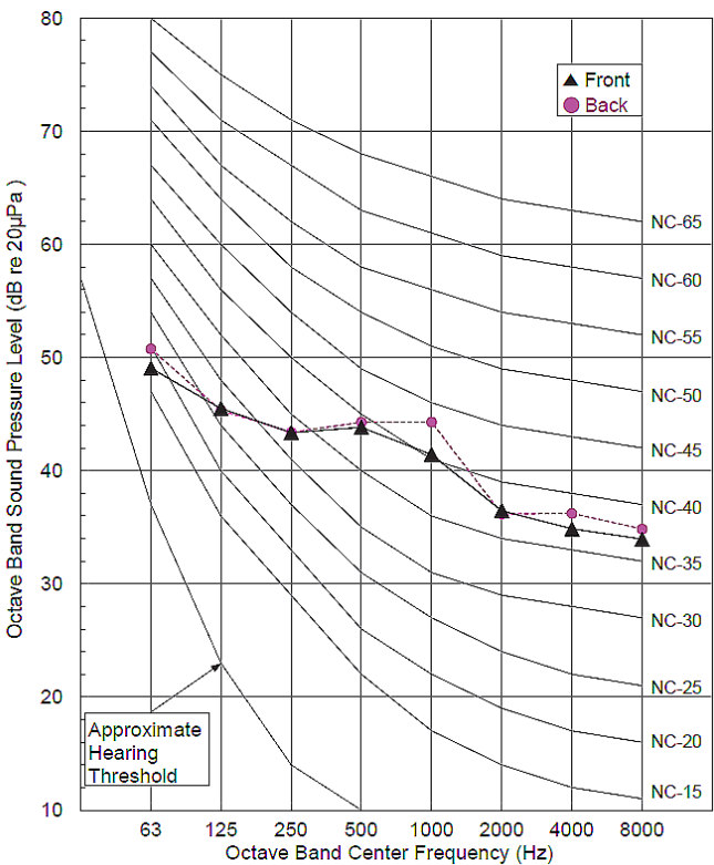
Figure 16: LSU090/120HSV5 Heating Sound Pressure Level Diagram.
