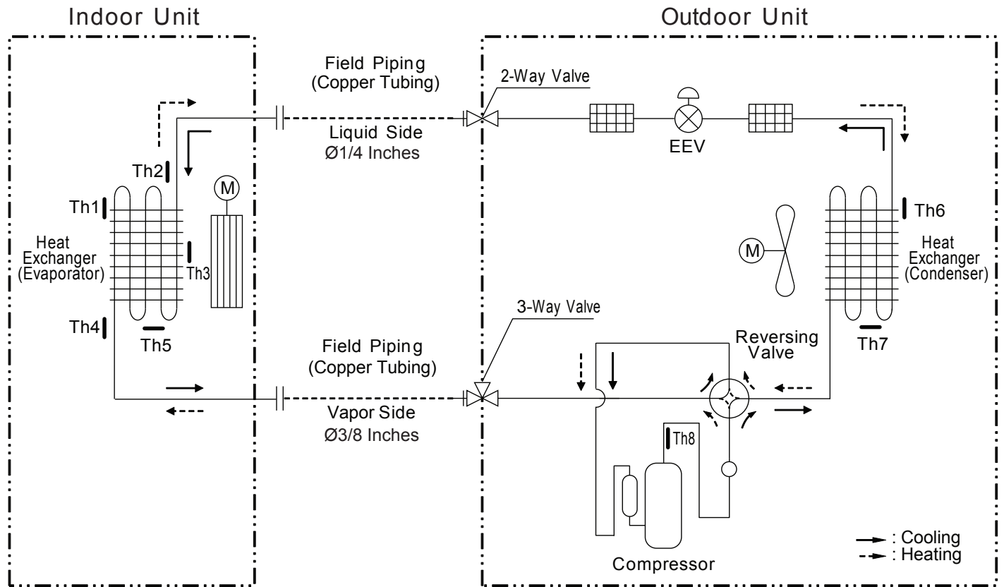
Figure 19: Refrigerant Flow Diagram for LA090HSV5, LA120HSV5 Units.
