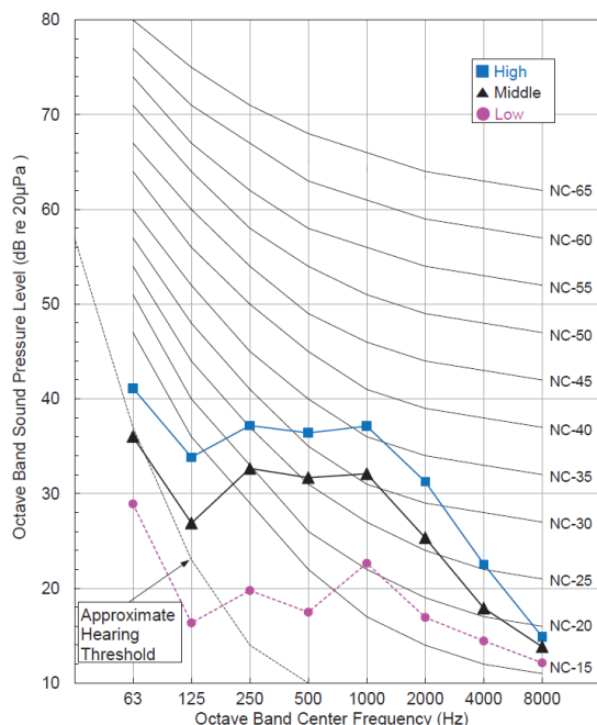
Figure 10: LAN090/120HSV5 Cooling Sound Pressure Level Diagram.
