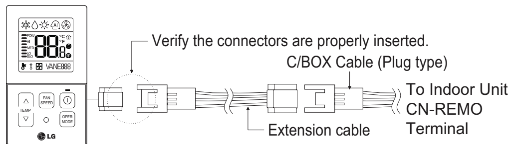
Figure 30: Wired Controller Connection on the Indoor Unit Terminal Block.
