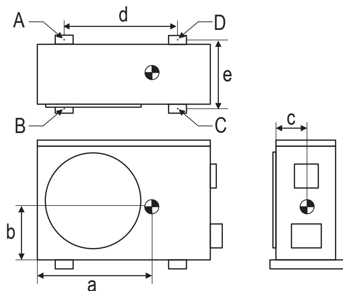
Figure 8: LSU090-120-181HSV5 Outdoor Unit Corner Weight and Center of Gravity Dimensions.
