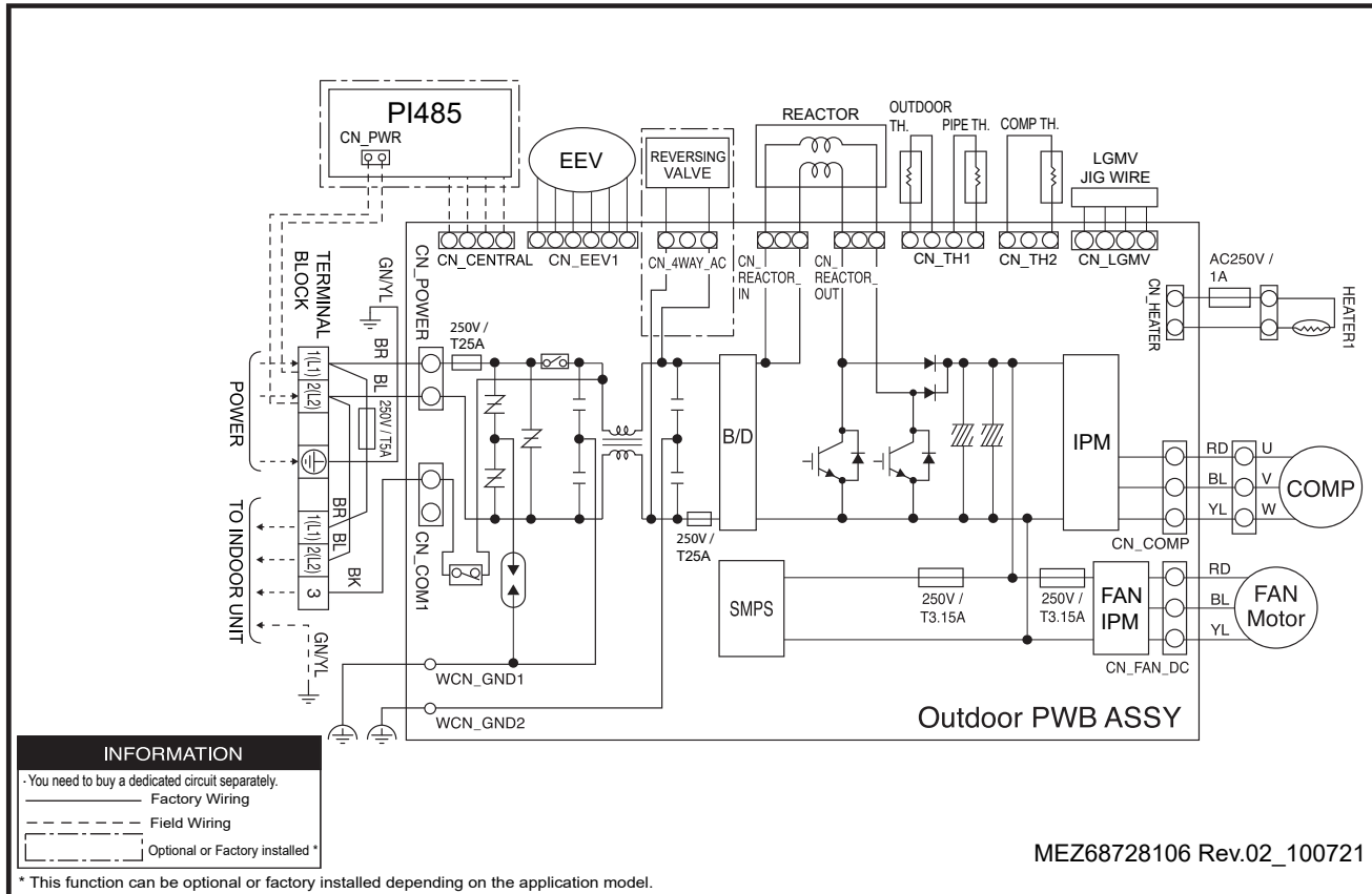
Figure 23: Wiring Diagram for LSU181HSV5 Units.
