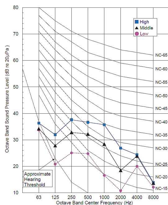
Figure 11: LAN090/120HSV5 Heating Sound Pressure Level Diagram.
