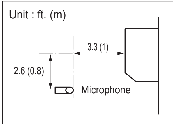
Figure 9: Art Cool Mirror Indoor Unit Sound Level Measurement.
