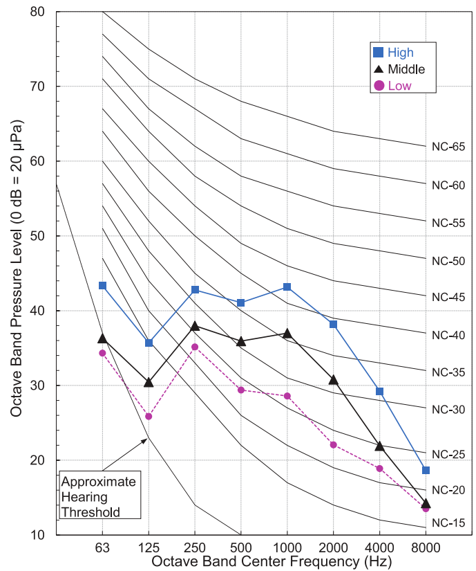
Figure 13: LAN181HSV5 Heating Sound Pressure Level Diagram.
