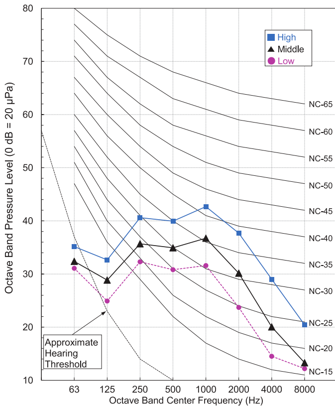
Figure 12: LAN181HSV5 Cooling Sound Pressure Level Diagram.
