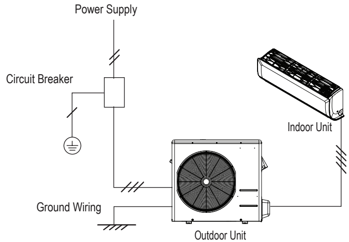
Figure 25: LA181HSV5 General Power / Communications System Schematic.
