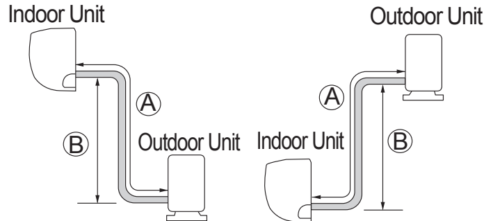
Figure 46: Single Zone Art Cool Mirror Wall Mount System Layout.
