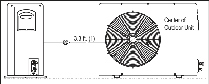
Figure 14: Outdoor Unit Sound Level Measurement.
