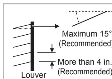
Figure 42: Louver Recommendations.
