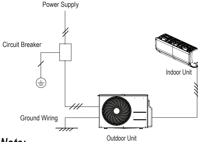
Figure 24: LA90HSV5 and LA120HSV5 General Power / Communications System Schematic.
