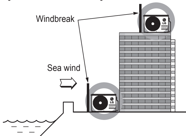
Figure 39: Oceanside Placement Using Windbreak.
