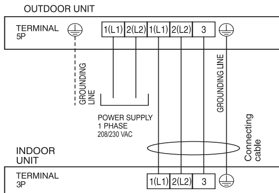
Figure 26: LA090-120HSV5 System Electrical Connections.
