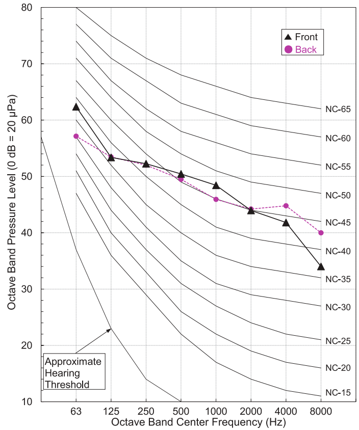
Figure 18: LSU181HSV5 Heating Sound Pressure Level Diagram.
