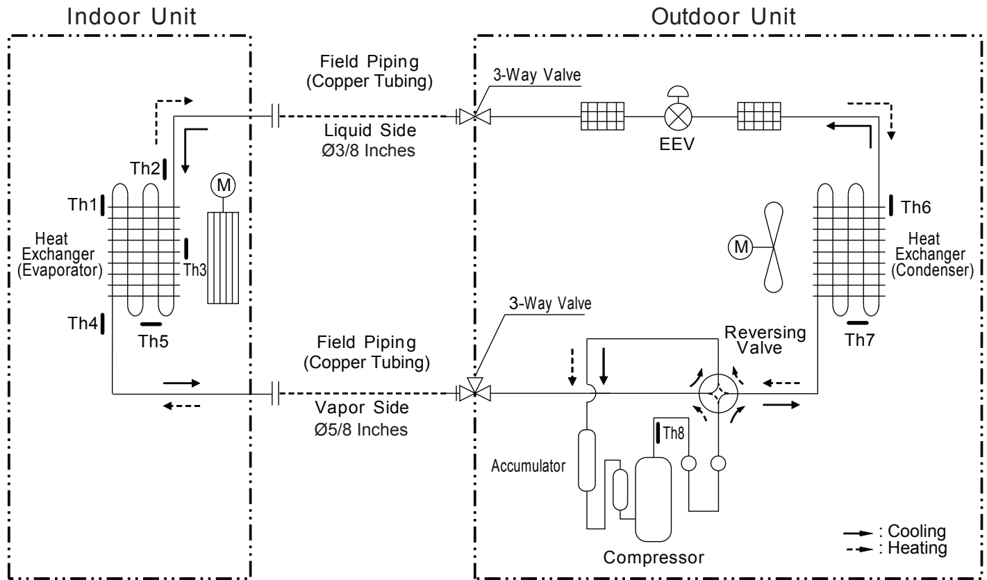
Figure 20: Refrigerant Flow Diagram for LA181HSV5 Units.
