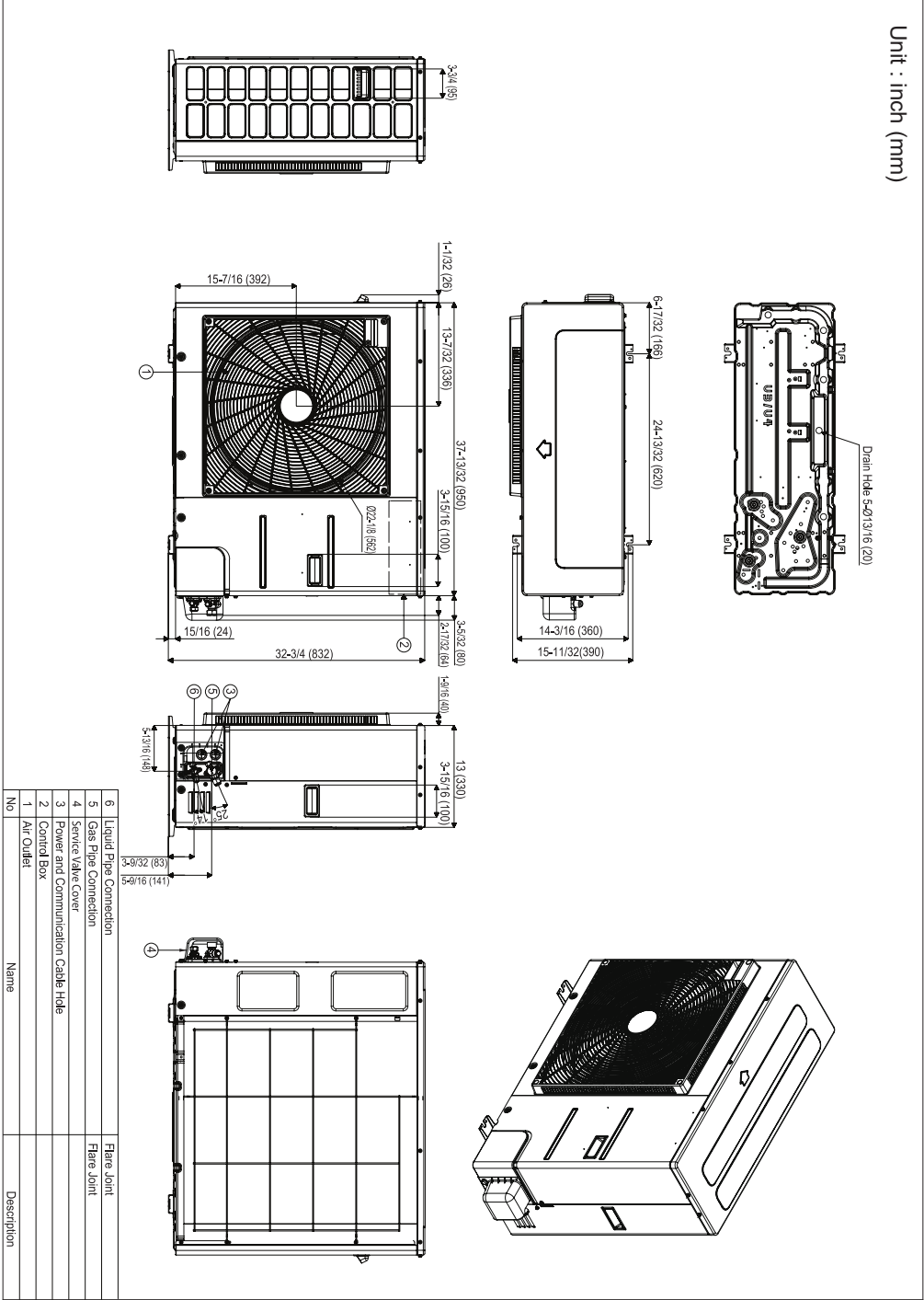
Figure 7: LSU181HSV5 Outdoor Unit Dimensions.
