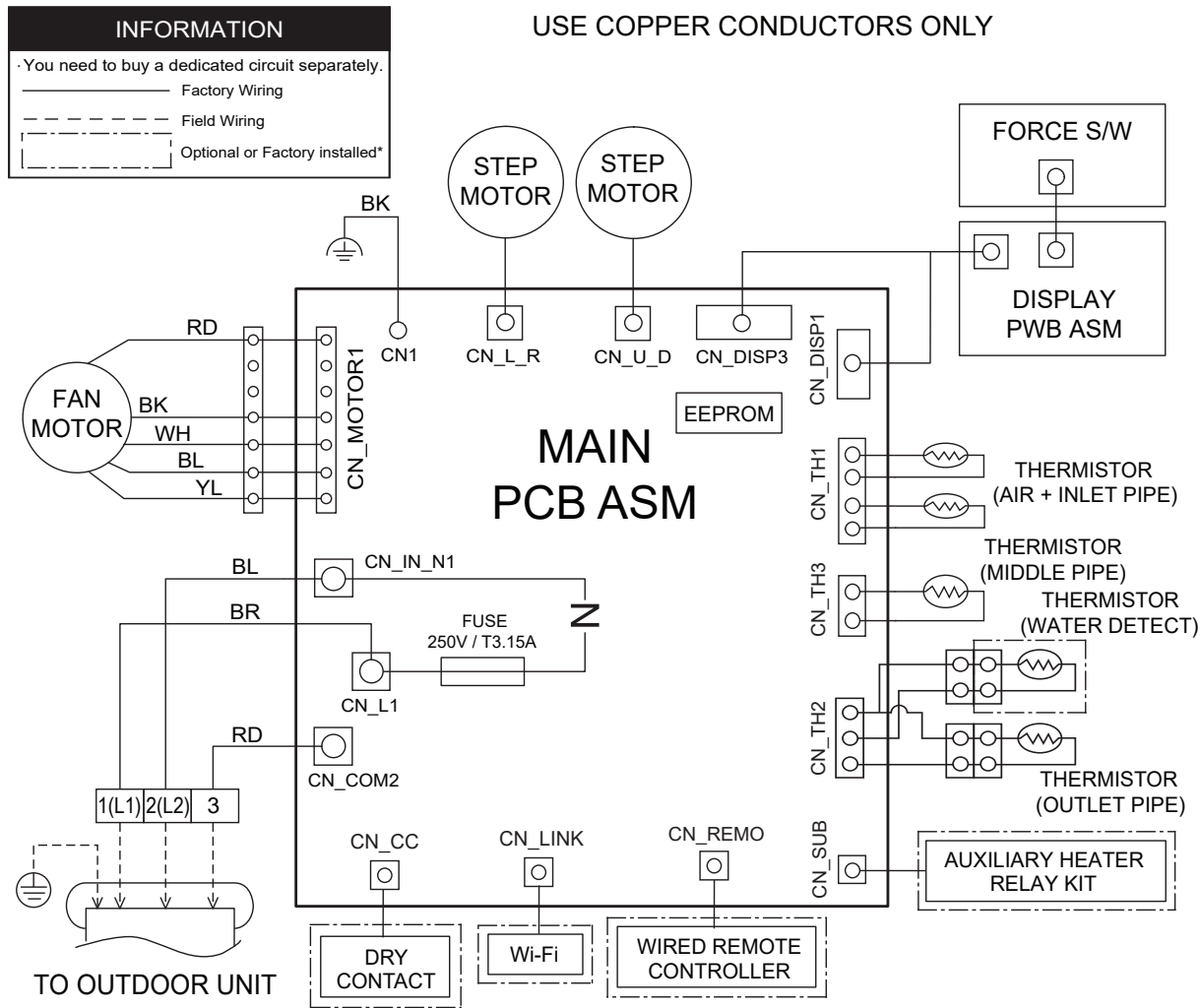
Figure 21: Wiring Diagram for LAN090HSV5, LAN120HSV5, LAN181HSV5 Units.
