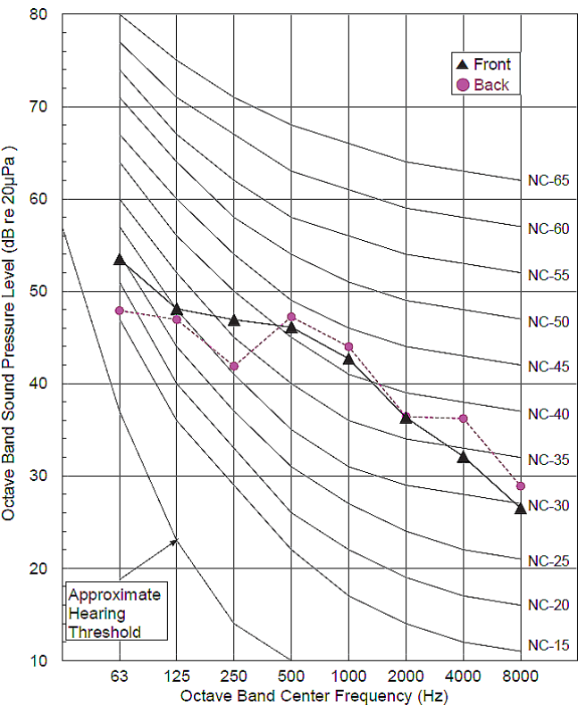
Figure 15: LSU090/120HSV5 Cooling Sound Pressure Level Diagram.
