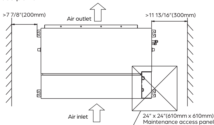
Maintenance access panel
