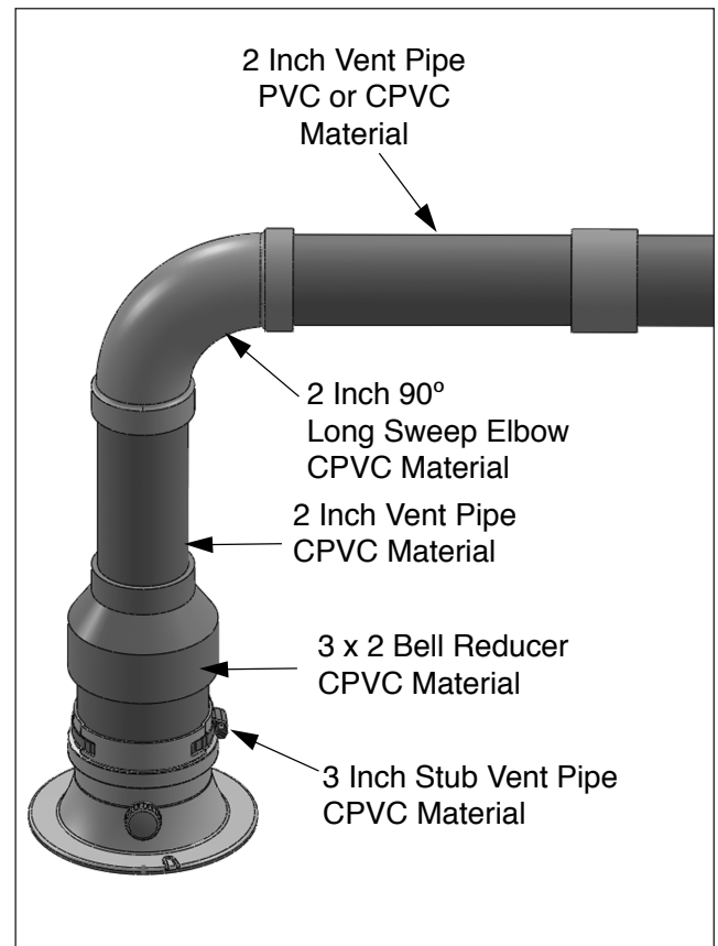
Fig. 21 - 2" CPVC/PVC Venting System Horizontal
