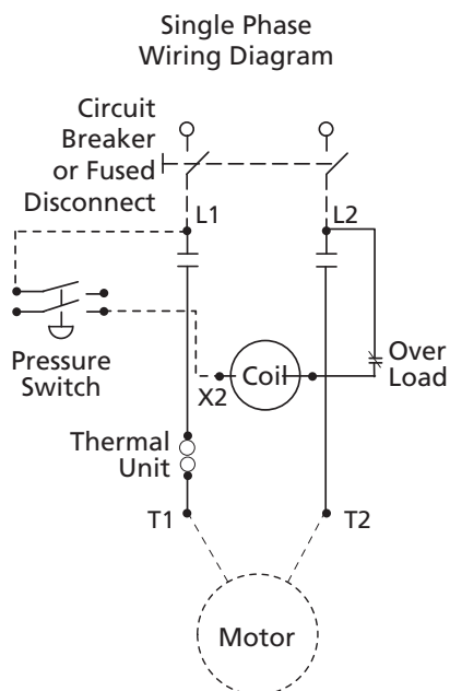
Figure 6 - For Motor Frame Sizes 184T, 215T, 254T or 284T. Refer to Motor Nameplate
