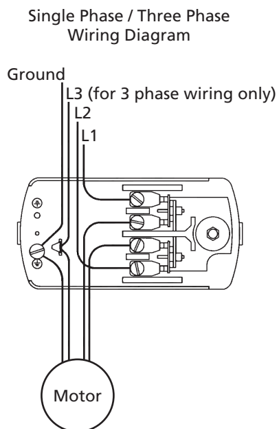
Figure 5 - For Motor Frame Sizes R56HZ, Y56Y or L143T. Refer to Motor Nameplate
