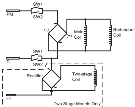
WIRING DIAGRAM - HSI MODELS 36H2X & 36H5X
