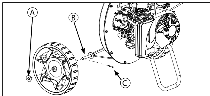
FIGURE 2 - Installing the Wheels
