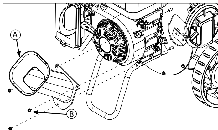
FIGURE 3 - Installing the Chipper Cone
