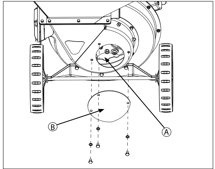
FIGURE 9- Inspect / Rotate Shredding Hammers A. J-Hammer Wear Area B. Access Panel
