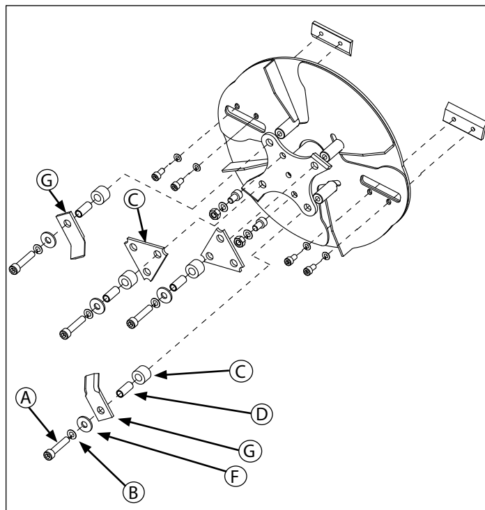
FIGURE 14- Rotor Housing
