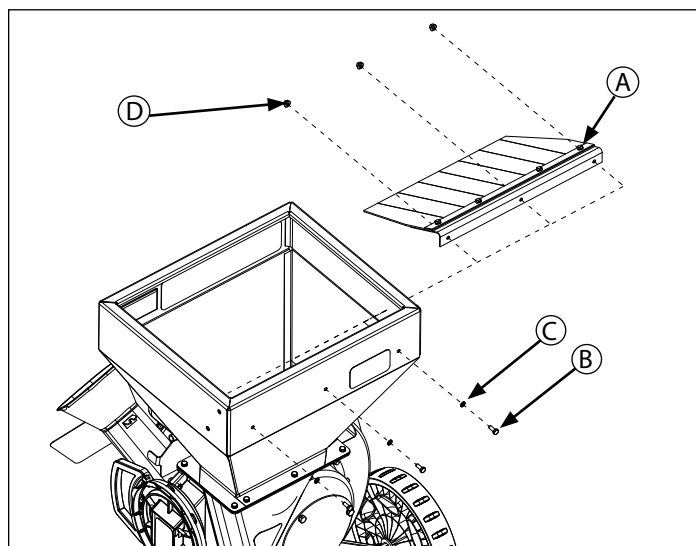
FIGURE 4 - Installing the Hopper Guard
