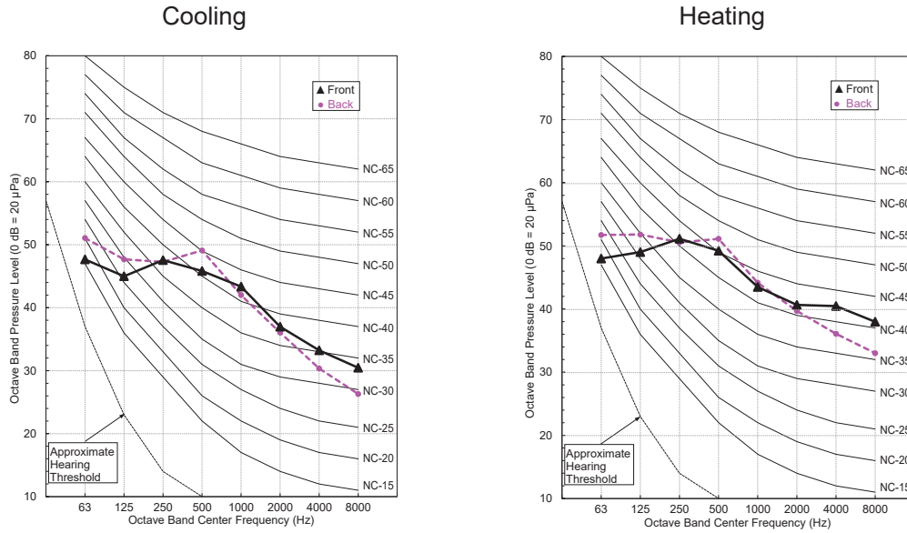
Figure 16: Sound Pressure Levels for LSU090HXV2 Outdoor Units.
