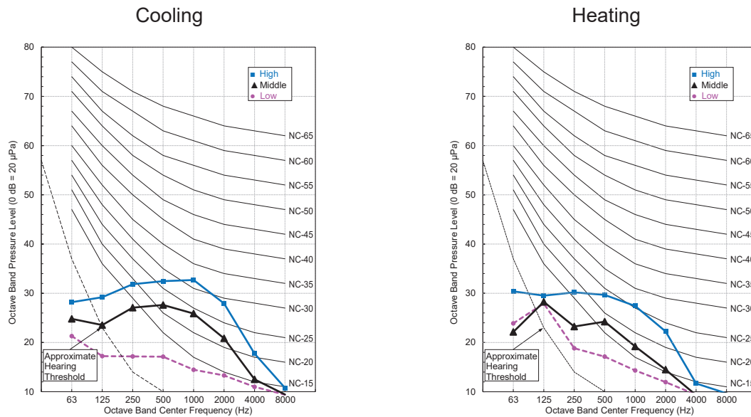
Figure 10: Sound Pressure Levels for LSN120HXV2 Indoor Units.
