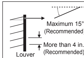
Figure 37: Louver Recommendations.
