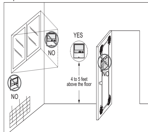
Figure 25: Proper Location for the Wired Controller.
