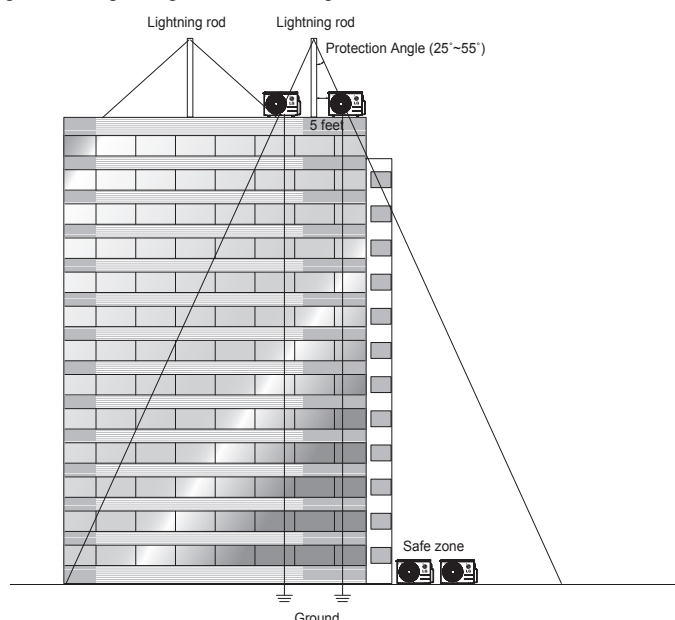
Figure 33: Lightning Protection Diagram.
