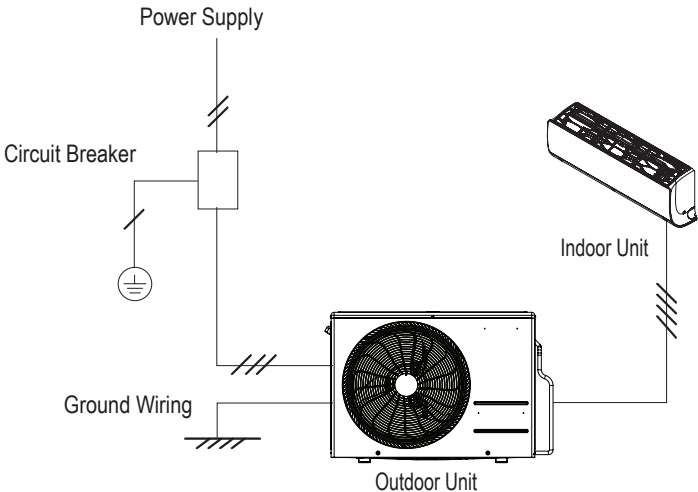
Figure 20: LS180HEV2, LS240HEV2, LS180HFV3, LS240HFV3 General Power / Communications System Schematic.
