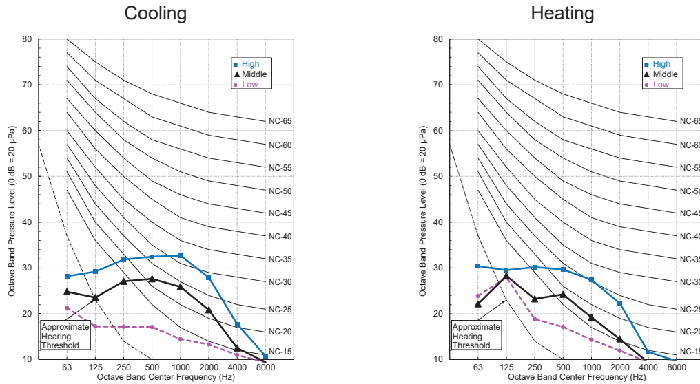
Figure 9: Sound Pressure Levels for LSN090HXV2 Indoor Units.
