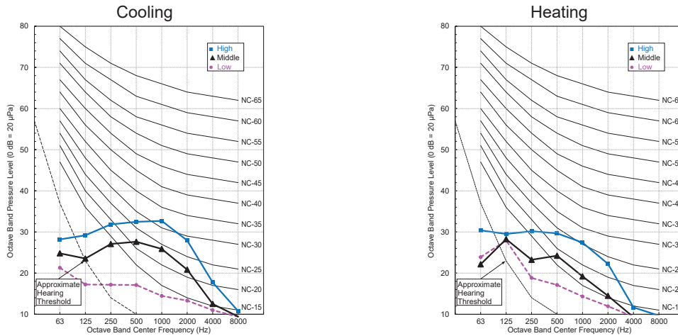
Figure 6: Sound Pressure Levels for LSN120HEV2, LSN120HFV3 Indoor Units.
