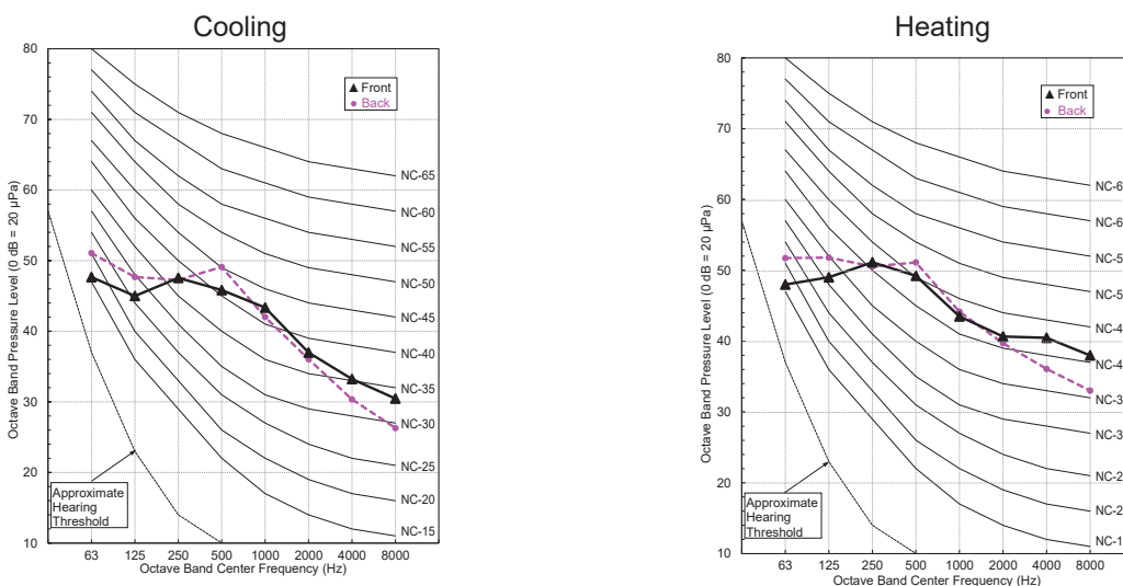
Figure 12: Sound Pressure Levels for LSU090HEV2, LSU090HFV3 Outdoor Units.
