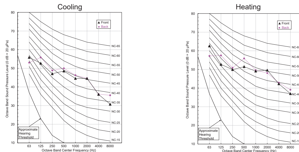
Figure 15: Sound Pressure Levels for LSU240HEV2, LSU240HFV3 Outdoor Units.
