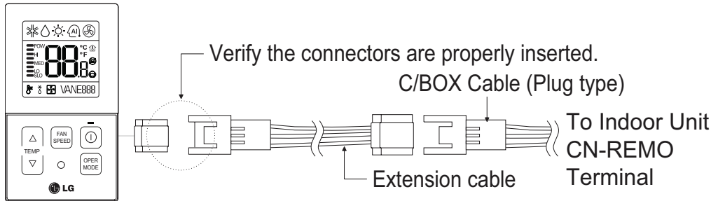
Figure 26: PZCWRC1 LG Wired Remote Extension Cable.
