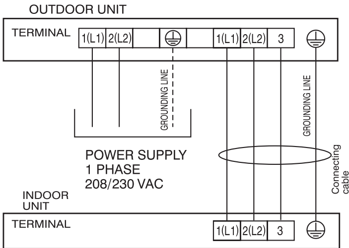
Figure 21: Terminal Block Wiring Diagram LS180HEV2, LS240HEV2, LS180HFV3, LS240HFV3
