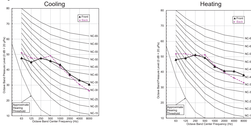
Figure 14: Sound Pressure Levels for LSU180HEV2, LSU180HFV3 Outdoor Units.
