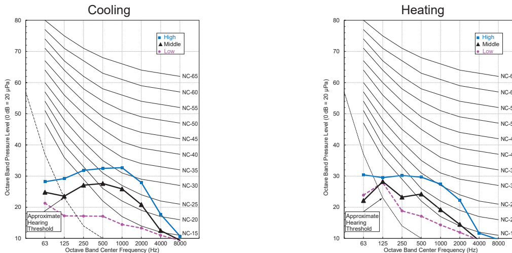
Figure 5: Sound Pressure Levels for LSN090HEV2, LSN090HFV3 Indoor Units.
