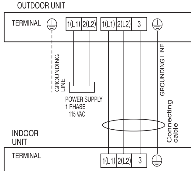
Figure 23: Terminal Block Wiring Diagram LS090HXV2, LS120HXV2
