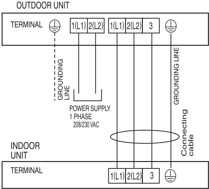
Figure 19: Terminal Block Wiring Diagram LS090HEV2, LS120HEV2, LS090HFV3, LS120HFV3
