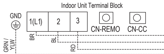
Figure 27: Wired Controller Connection on the Indoor Unit Terminal Block (Appearances and Terminal Placement Will Vary Depending on Model).
