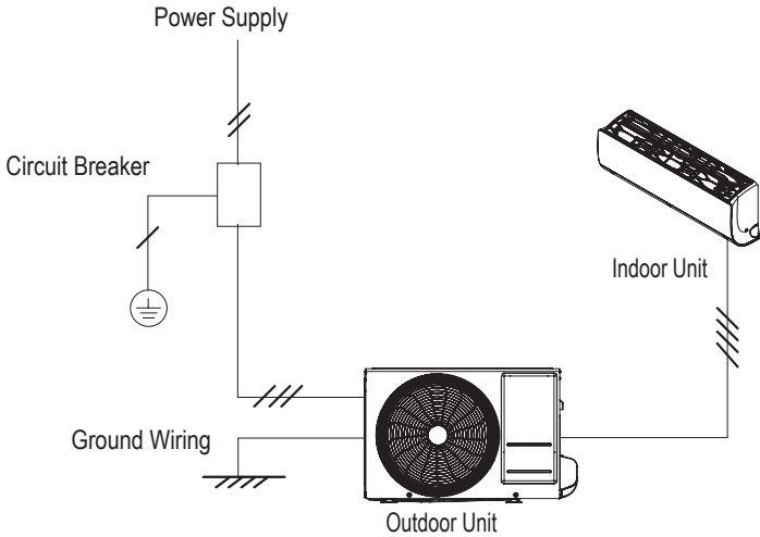
Figure 18: LS090HEV2, LS120HEV2, LS090HFV3, LS120HFV3 General Power / Communications System Schematic.
