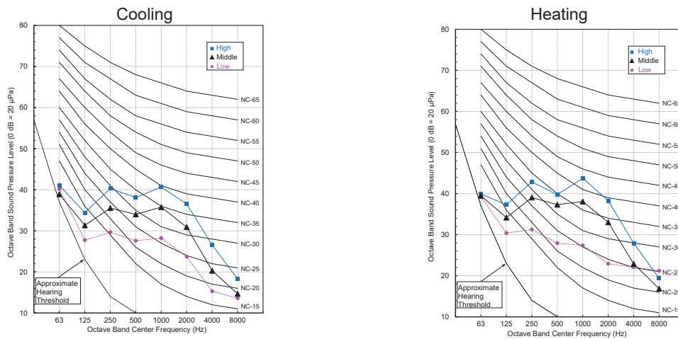
Figure 8: Sound Pressure Levels for LSN240HEV2, LSN240HFV3 Indoor Units.
