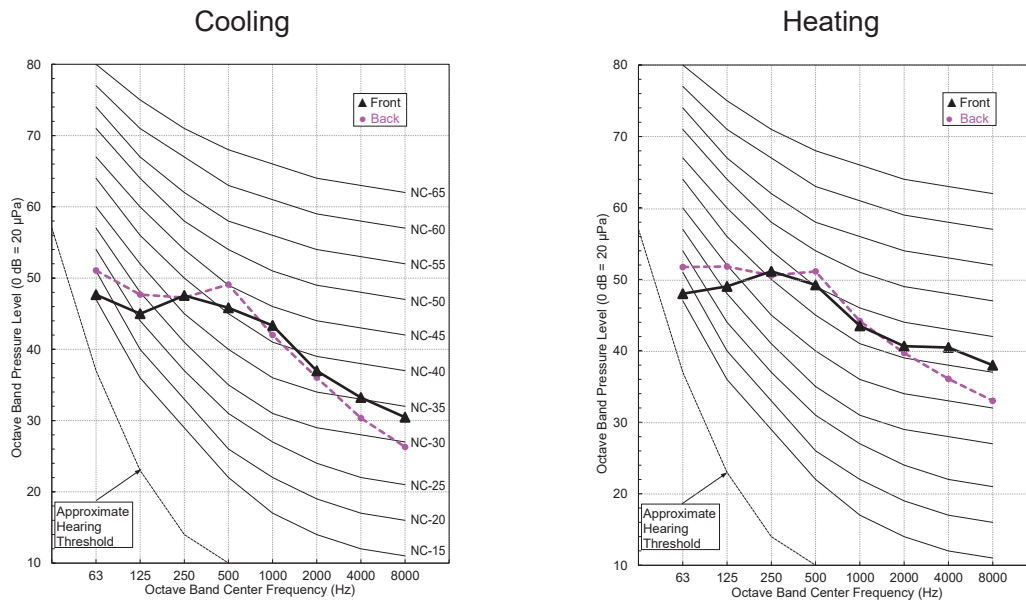
Figure 17: Sound Pressure Levels for LSU120HXV2 Outdoor Units.
