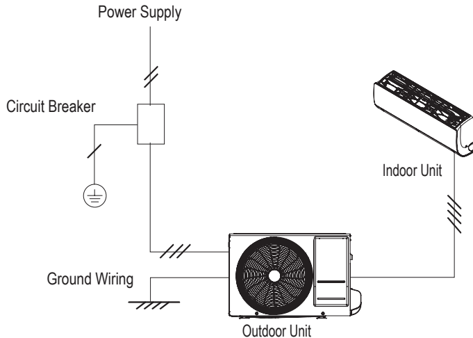
Figure 22: LS090HXV2 and LS120HXV2 General Power / Communications System Schematic.
