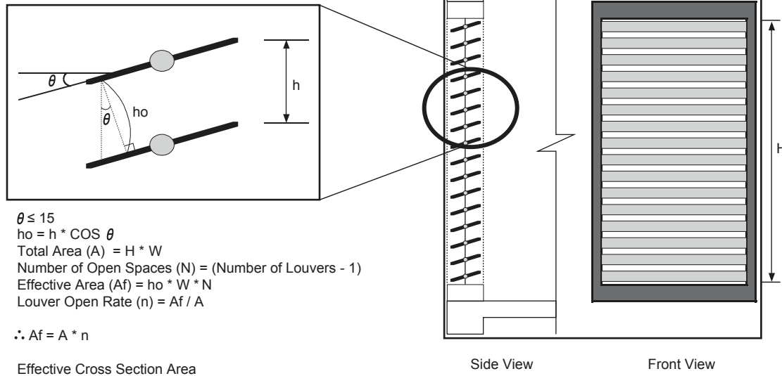
Figure 40: Example of Installing Outdoor Unit Indoors.
