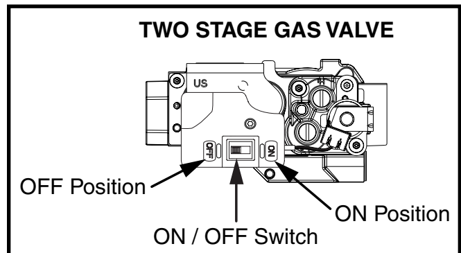
Figure 2. Gas Valve
