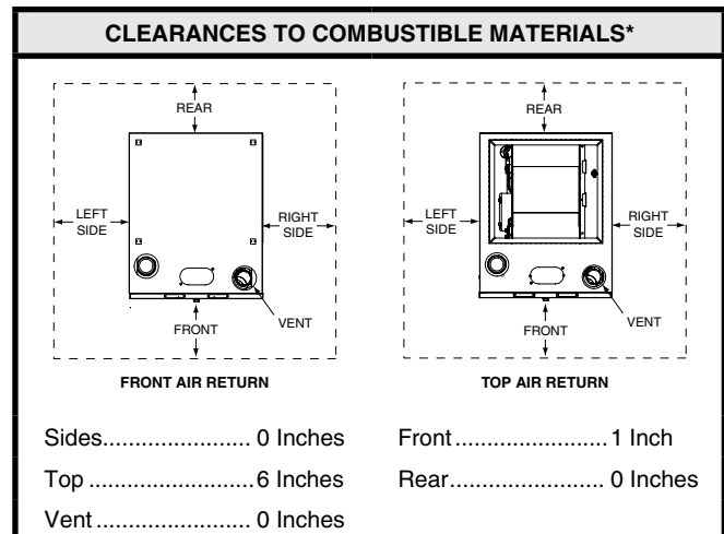
Figure 1. Minimum Clearances
