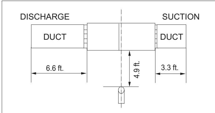
Figure 17: Mid Static Ducted Indoor Unit Sound Pressure Level Measurement Location.
