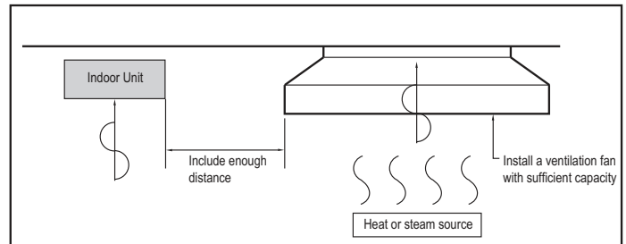
Figure 21: Installing Near a Heat or Steam Source.
