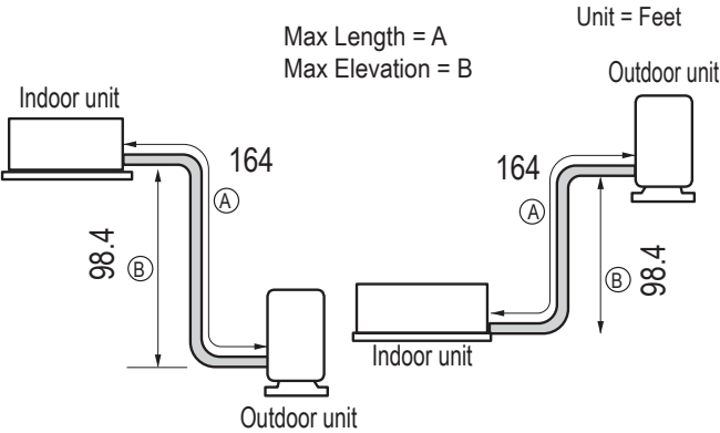
Figure 40: Typical KSUJA181A, KSUJA241A System Layout.
