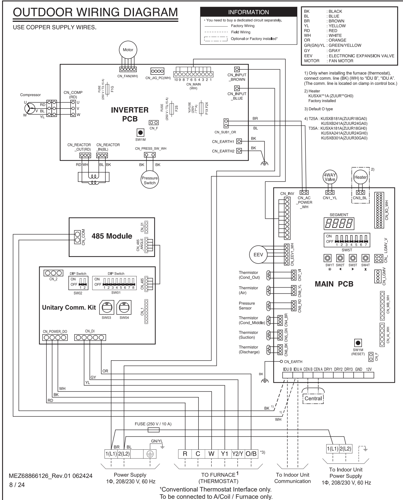
Figure 50: KUSXA181A, KUSXA241A Outdoor Units Wiring Diagram.
