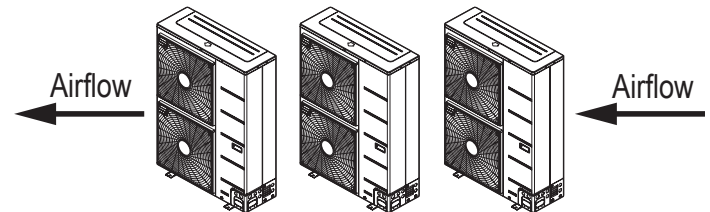
Figure 29: Improper Outdoor Unit Placement.
