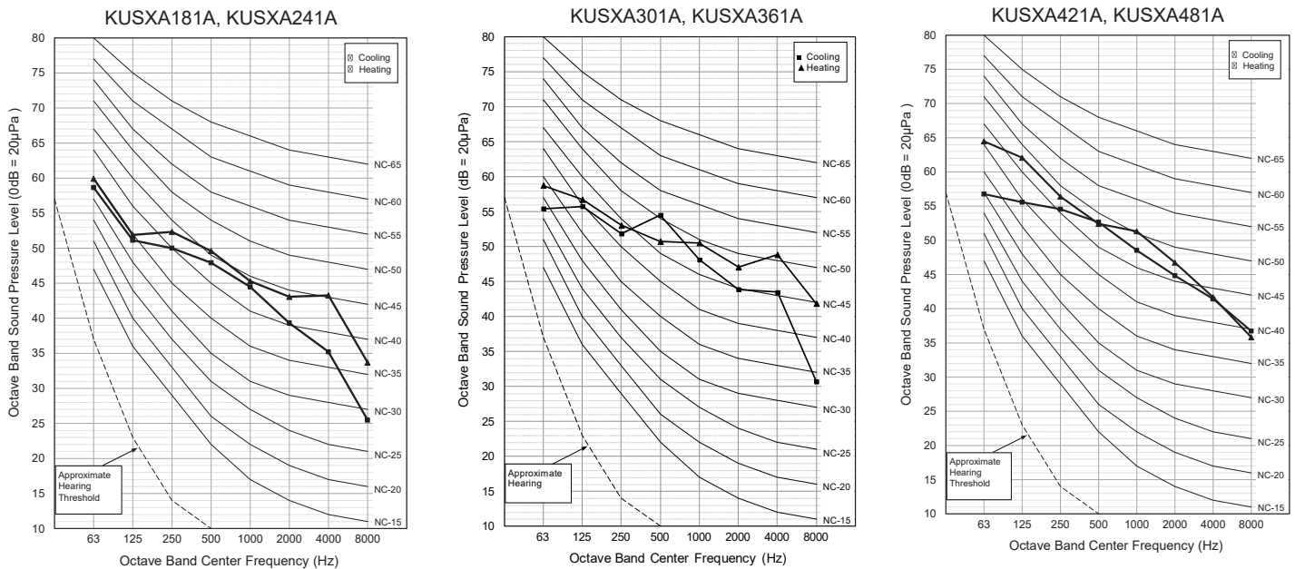
Figure 15: Mid Static Ducted LGRED° Outdoor Unit Sound Pressure Level Diagrams.
