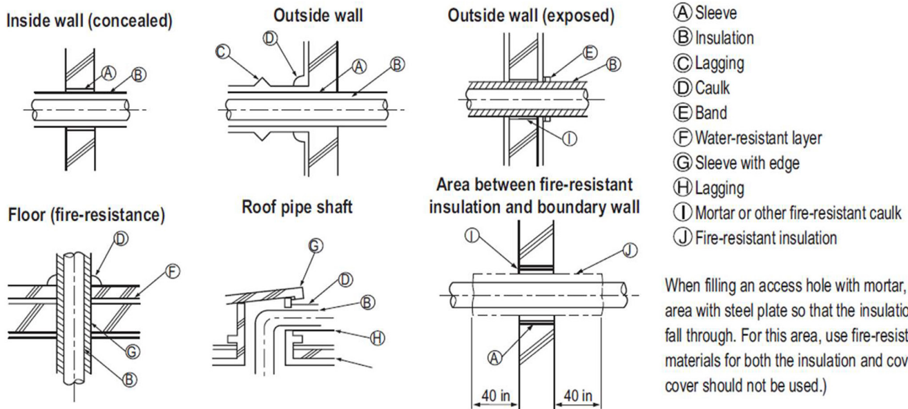
Figure 47: Pipe Sleeve Options.
