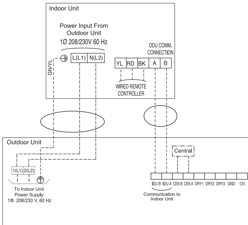
Figure 61: Single Zone Power / Communication System Diagram (Appearances May Vary).
