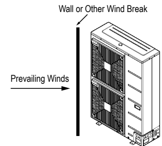
Figure 25: Wind Break.
