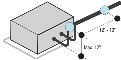
Figure 46: Pipe Support at Indoor Unit.
