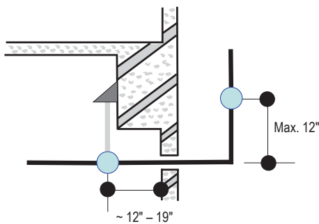
Figure 45: Typical Pipe Support Location—Change in Pipe Direction.
