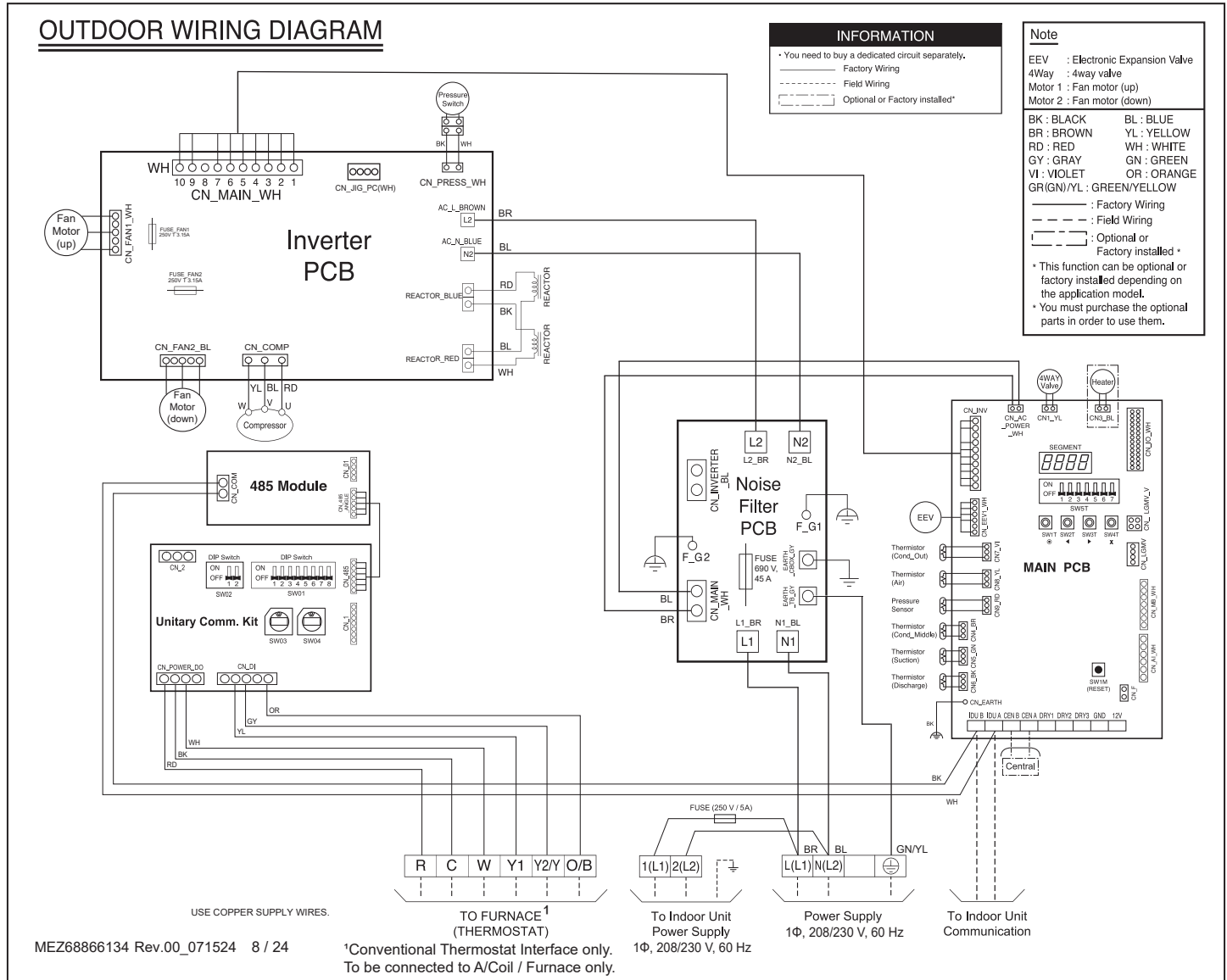
Figure 51: KUSXA301A, KUSXA361A Outdoor Units Wiring Diagram.
