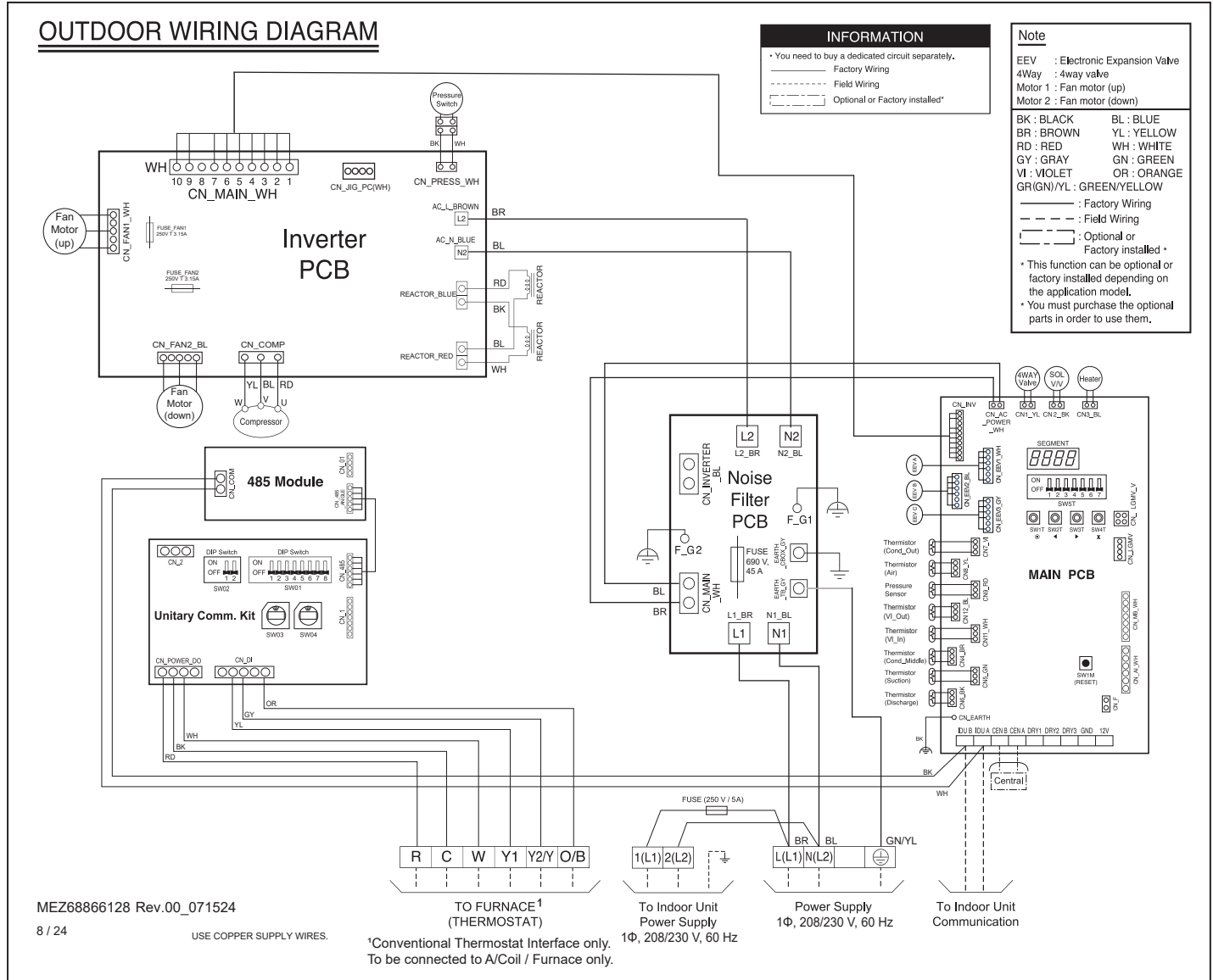
Figure 52: KUSXA421A, KUSXA481A Outdoor Units Wiring Diagram.
