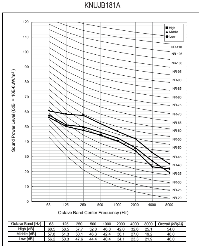
Figure 20: Mid Static Ducted Indoor Unit Sound Power Level Diagrams.
