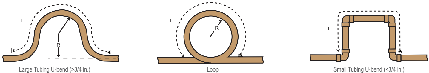
Figure 42: Coiled Expansion Loops and Offsets (Plan View).
