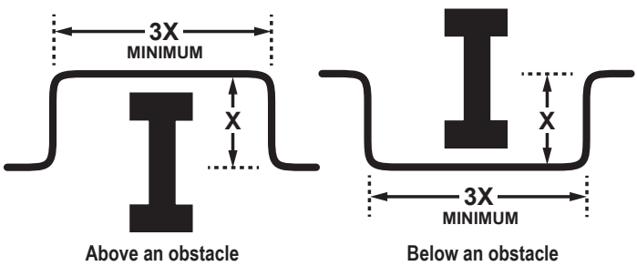
Figure 43: Installing Piping Above and Below an Obstacle.
