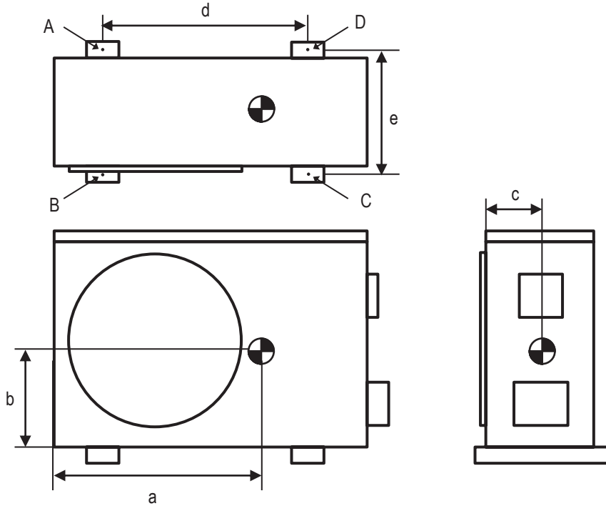
Figure 10: Center of Gravity and Corner Weight Dimensions Diagram.
