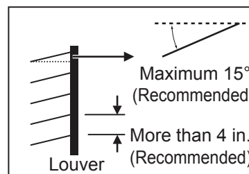
Figure 33: Louver Recommendations.
