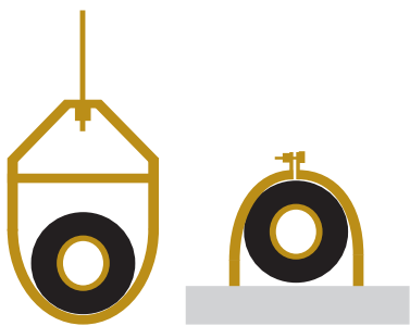
Figure 44: Pipe Hanger Details.
