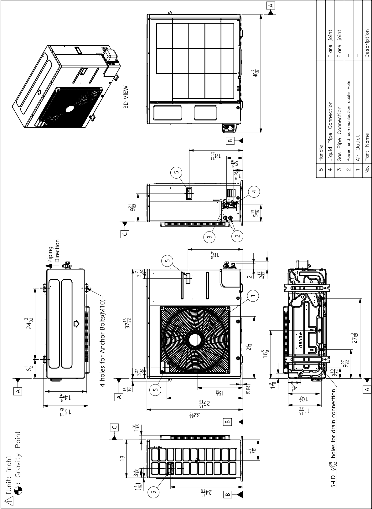
Figure 8: KUSXA181A, KUSXA241A, KUSXA301A Outdoor Unit Dimensions.
