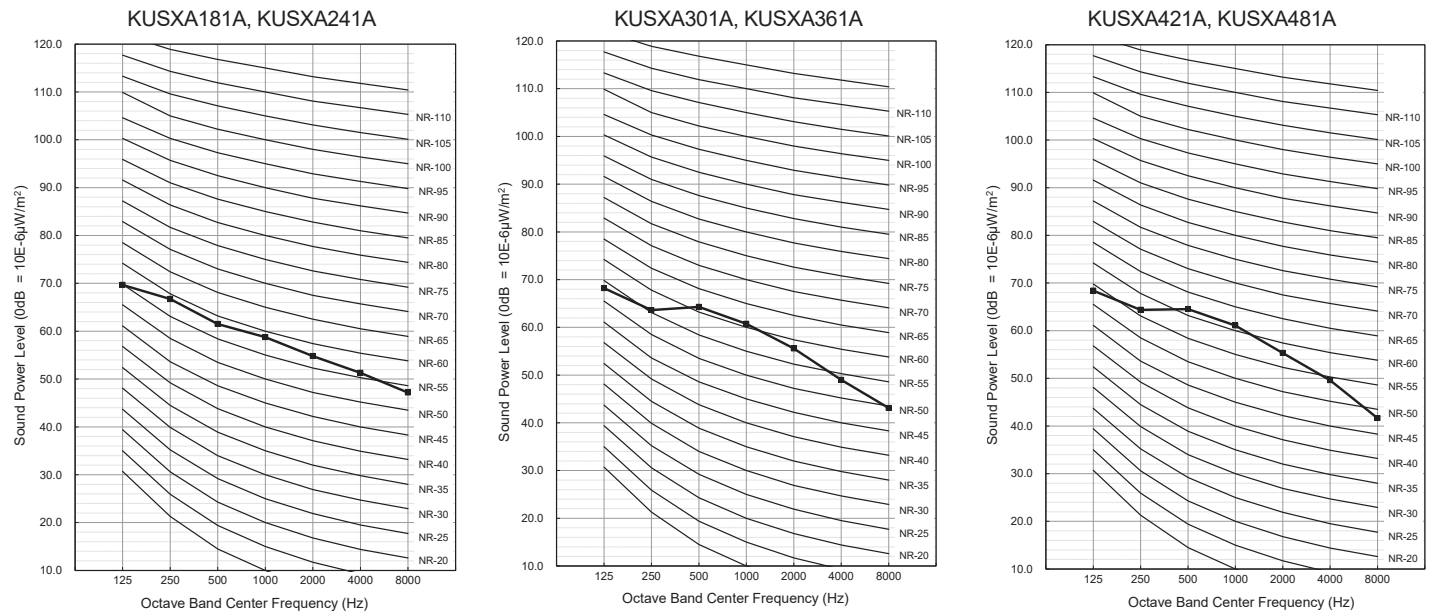
Figure 16: Mid Static Ducted LGRED° Outdoor Unit Sound Power Level Diagrams.
