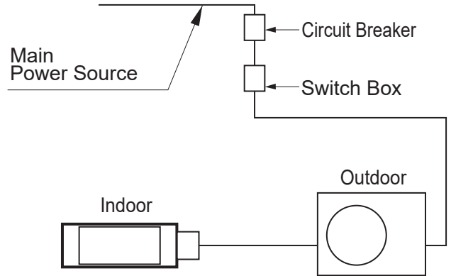
Figure 58: Power Wiring Example
