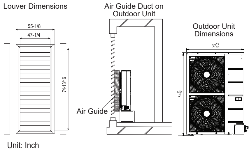
Figure 35: Example of Installing Outdoor Unit Indoors.
