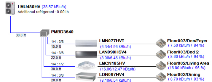
Figure 2: Example of a LATS Tree Diagram.
