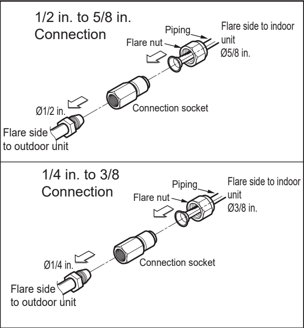
Figure 38: KNUJB181A Mid-Static Ducted Indoor Unit Refrigerant Pipe Connections.
