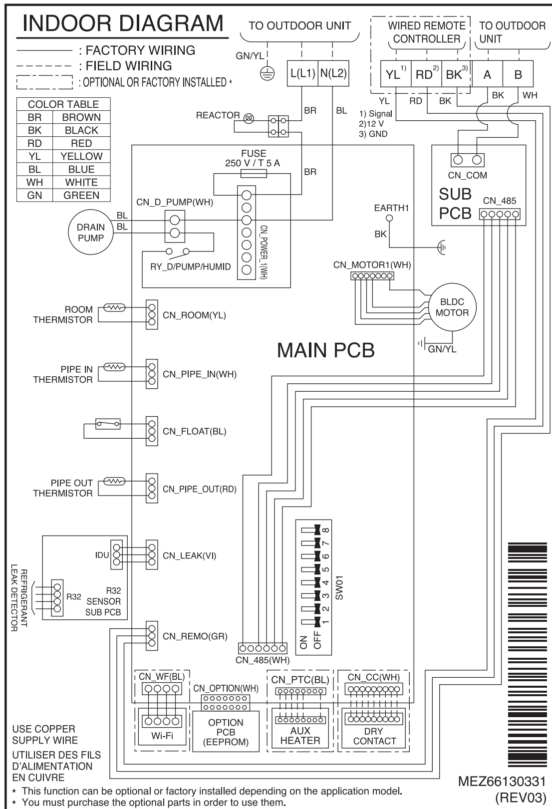
Figure 54: KNUJB301A, KNUJB361A, KNSJB421A, KNSJB481A Indoor Units Wiring Diagram.
