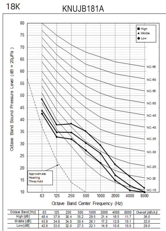
Figure 18: Mid Static Ducted LGRED® Indoor Unit Sound Pressure Level Diagrams.
