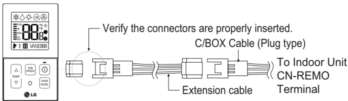
Figure 62: PZCWRC1 LG Wired Remote Extension Cable.
