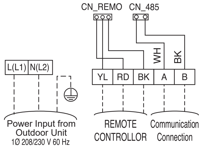
Figure 63: Wired Controller Connection (Example Only).
