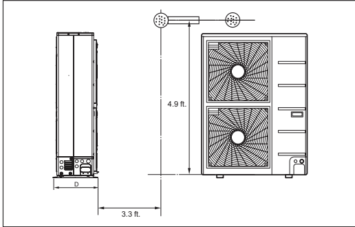
Figure 14: Mid Static Ducted LGRED° Outdoor Unit Sound Pressure Level Measurement Location.
