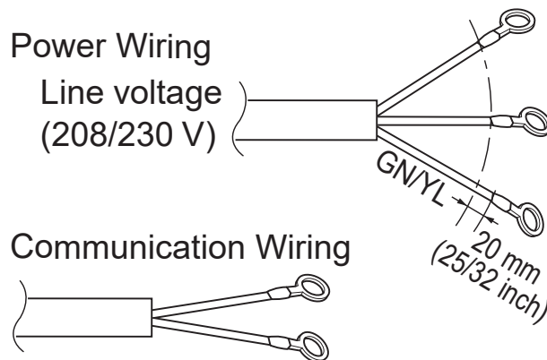
Figure 60: Single Zone Outdoor Unit to Indoor Unit Wiring and Communications Cable Diagram.
