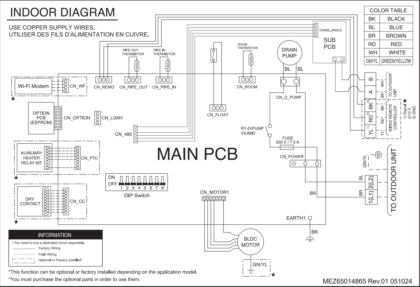
Figure 53: KNUJB181A , KNUJB241A Indoor Units Wiring Diagram.
