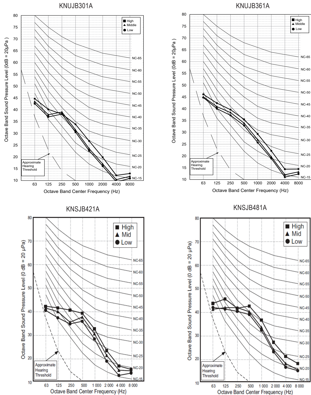
Figure 19: Mid Static Ducted LGRED° Indoor Unit Sound Pressure Level Diagrams.
