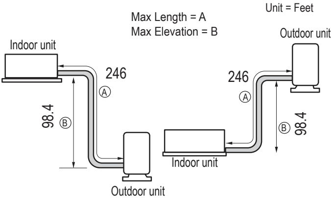
Figure 41: Typical KSUJA301A, KSUJA361A, KSSJA421A, and KSSJA481A System Layout.
