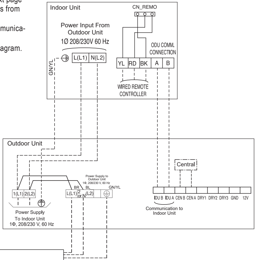
Figure 59: General Single Zone System Power / Communications System Schematic (Appearances May Vary)
