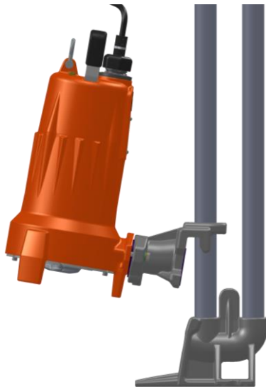
DISCONNECTED POSITION
