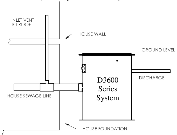
Figure A – Inlet Venting
