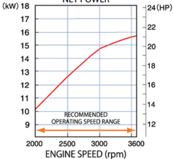
NET POWER
